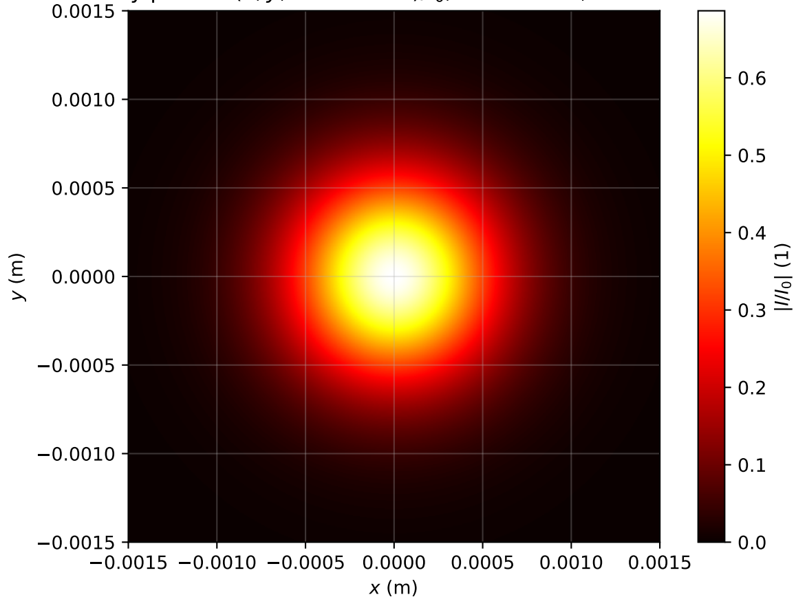
Intensity profile I(x, y, z = 2.149m)/I_0 , Pin=0.4Pcr, artificial time
